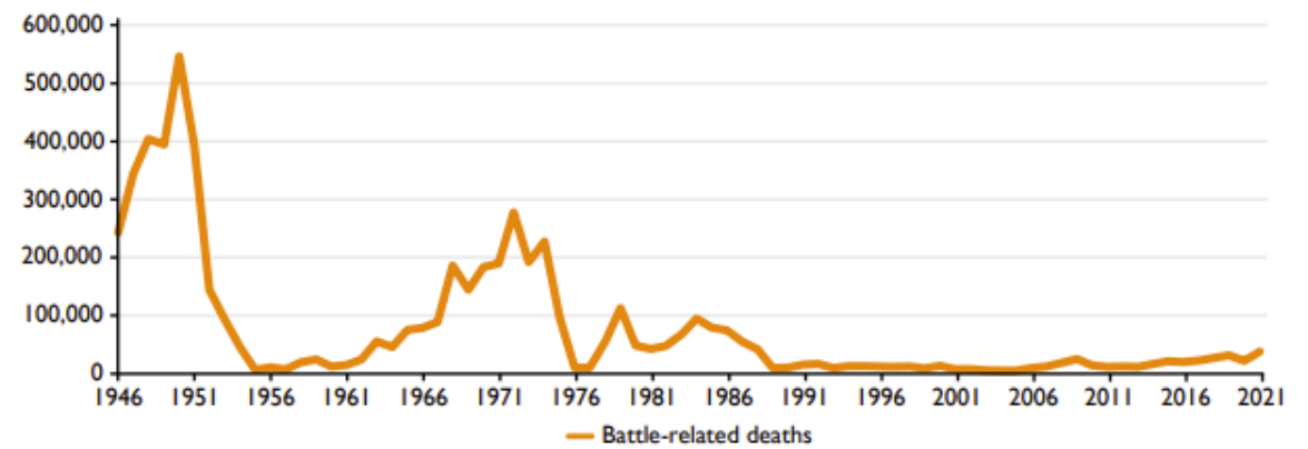
Figure 3: Battle-related deaths from state-based conflicts in Asia, 1989–2021 14
